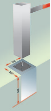
Fundament B6010/B7010/B8010 (mm)
