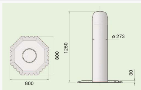
Measurements SafetyGuard 450TR (mm)
