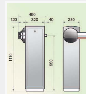
Dimensions B3000/B5010 (mm)
