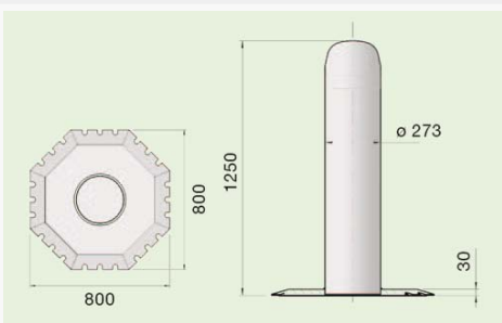
Measurements SafetyGuard 350 (mm)
