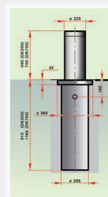
Dimensions/Foundation DK500/DK700 (mm)
