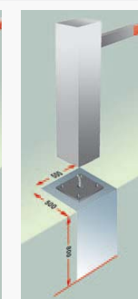
Foundation B3000/B5010 (mm)
