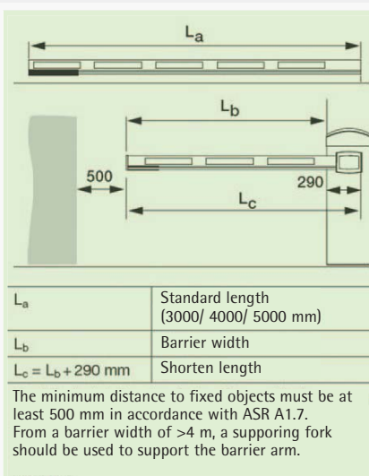
Barrier BS50
