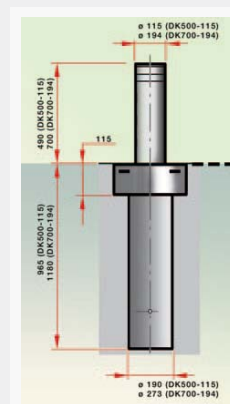
Dimensions/Foundation DK500-115/DK700-194 (mm)
