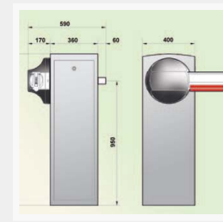
Dimensions B6010 (mm)
