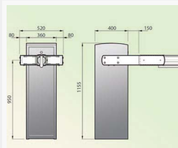
Dimensions B7010/B8010 (mm)
